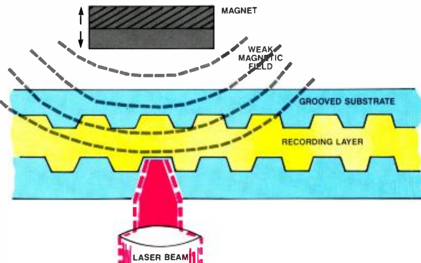
Figure 1. Simplified cross-section of a magneto-optical disc, showing alternating pattern of preformatted grooves in substrates of both sides of the disc. Whenever record laser is energized, recording layer is heated to a temperature at which the weak magnetic field affects its polarity. Magnet's polarity is inverted during erase mode.
