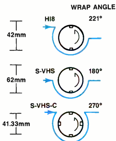
Figure 3. A comparison of Hi8, S-VHS and S-VHS-C tape wraps. The length of the video track and its angle across the tape are specific to each format and are related to the angle of tape-to-head contact. The head diameter and tape wrap difference between S-VHS and S-VHS-C requires additional heads to accommodate compatibility.
