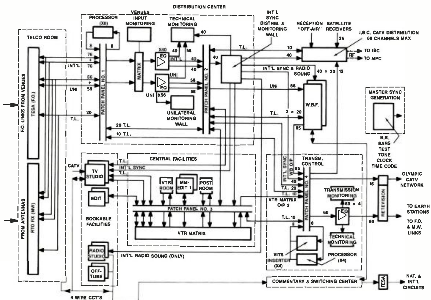
Figure 1. Signal-flow block diagram for the International Broadcast Center of the Barcelona Olympic Games. (Note that in the diagram, T.L. refers to tie lines; W.B.F. refers to "world broadcast feed;" 4-wire circuits refer to commentary and talkback feeds.)
