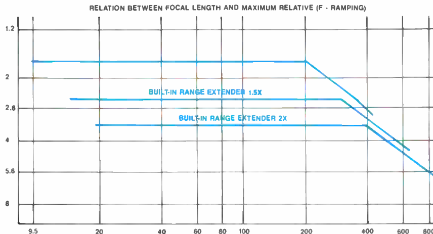
Figure 1. The chart illustrates the relation between focal length and maximum relative aperture — F-ramping for a modern lens. As the lens zooms in with the iris wide open, less light is passed through the lens.
